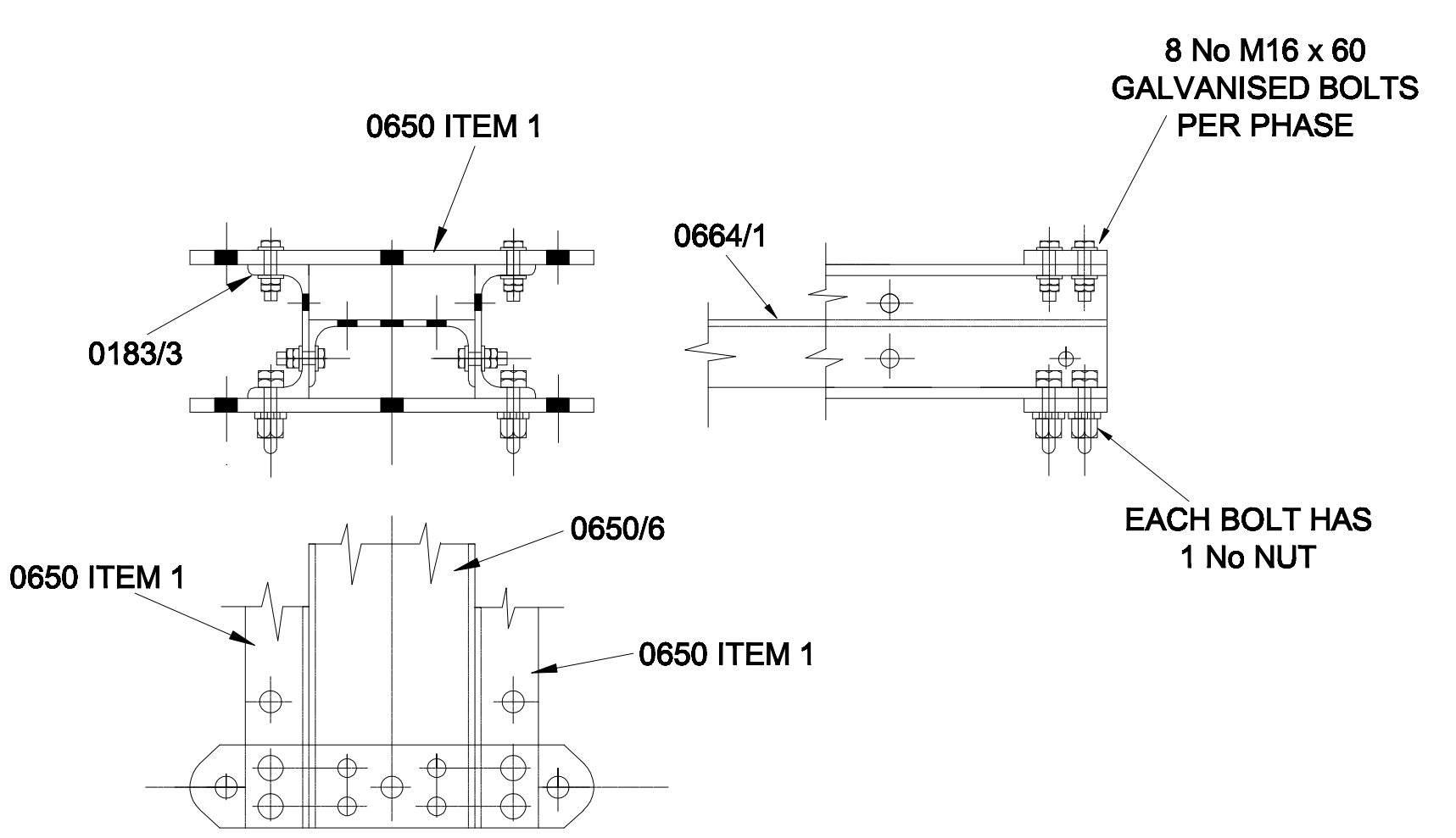
ENLARGED DETAIL ' A ' SCALE 1 : 7.5
